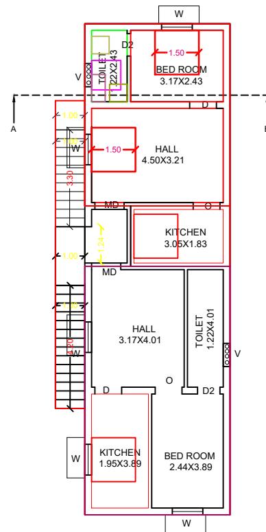
EXI & PRO.GROUND FLOOR PLAN
