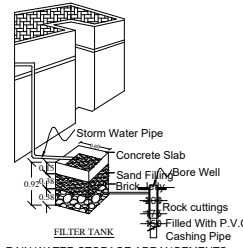
RAIN WATER STORAGE ARRANGEMENTS SCALE (1:50)
