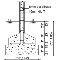
COLUMN FOUNDATION DETAIL SCALE (1:50)
