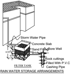
RAIN WATER STORAGE ARRANGEMENTS
