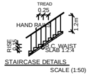
STAIRCASE DETAILS SCALE (1:50)
