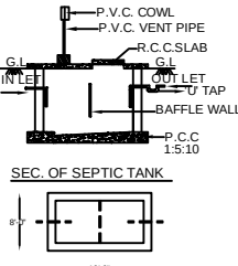
PLAN OF SEPTIC TANK SCALE (1:50)
