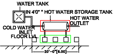
SOLAR HOT WATER SYSTEM DETAIL SCALE (1:50)
