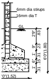
COLUMN FOUNDATION DETAIL SCALE (1:50)
