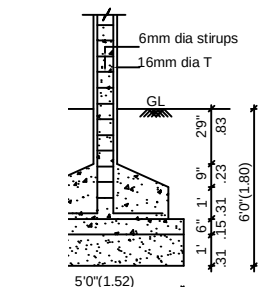
COLUMN FOUNDATION DETAIL SCALE (1:50)
