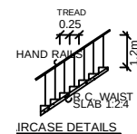
SCALE (1:50)
