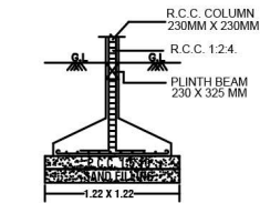
FOUNDATION DETAIL (NOT TO SCALE)
