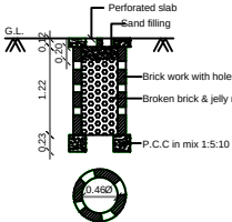
PERCOLATION PIT FOR 30 Sq. m.
