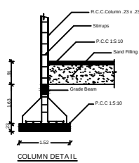
COLUMN DETAIL
