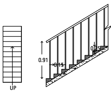
STAIRCASE DETAILS
