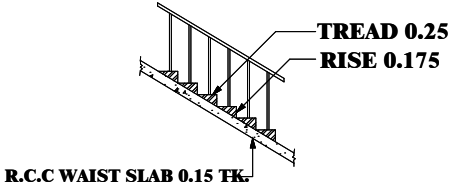
STAIR CASE DETAILS
