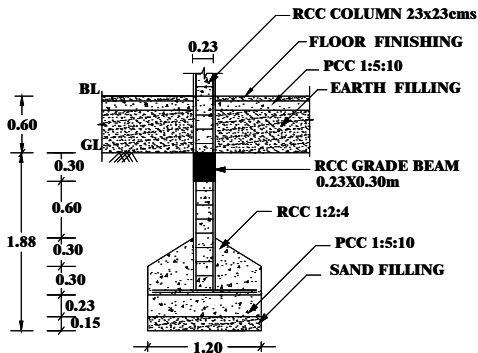
FOUNDATION DETAILS
