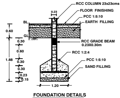
FOUNDATION DETAILS
