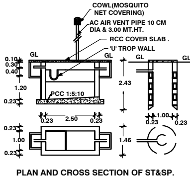
PLAN AND CROSS SECTION OF ST&P.
