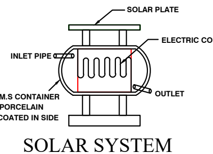
SOLAR SYSTEM
