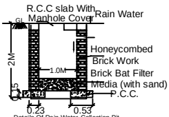
Details of Rain Water Collection Dr. (Recharge Well Method) SCALE: 1"=4'0"
