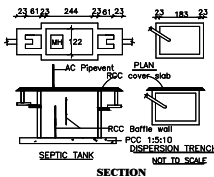
SECTION
