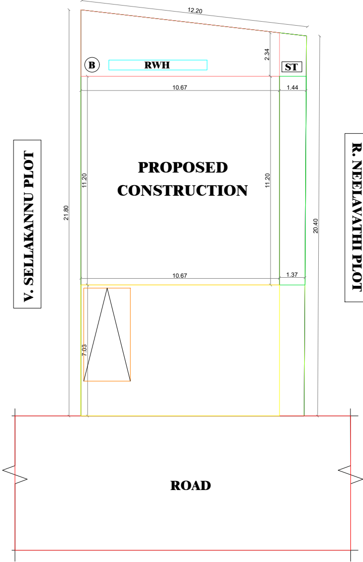
SITE PLAN - (1:100)
