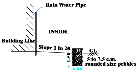
RAINWATER HARVESTING
