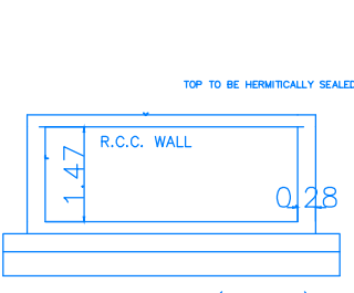
RWH_SECTION (SAMPLE)
