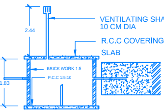
SEPTIC TANK DETAIL
