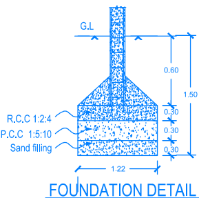
FOUNDATION DETAIL
