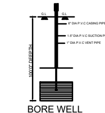
BORE WELL
