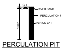
PERCOLATION PIT
