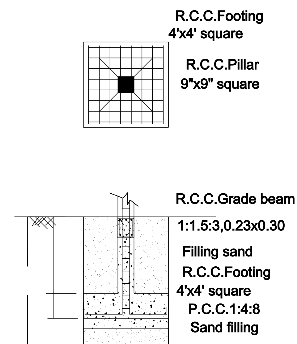
Foundation details Scale 1:50
