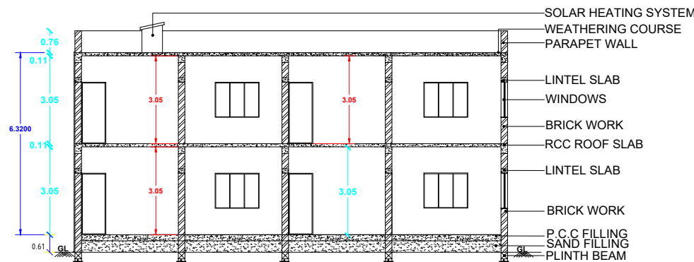
SECTION ON-SS
