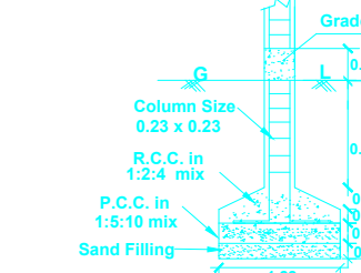
COLUMN DETAILS NOT TO SCALE
