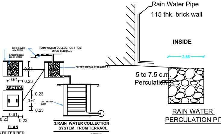
RAIN WATER COLLECTION SYSTEM FROM TERRACE
