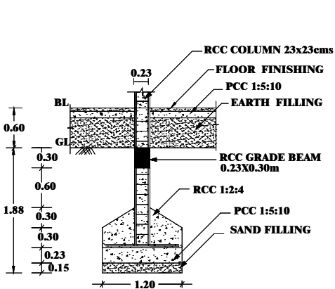
FOUNDATION DETAILS
