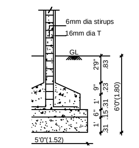
COLUMN FOUNDATION DETAIL SCALE (1:50)
