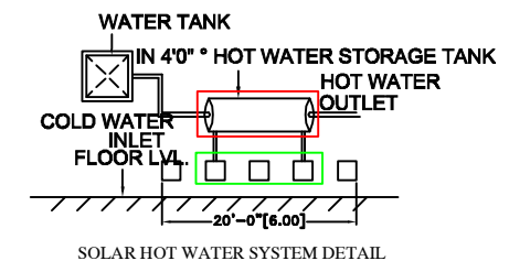
SOLAR HOT WATER SYSTEM DETAIL SCALE 1:100
