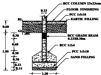
FOUNDATION DETAILS
