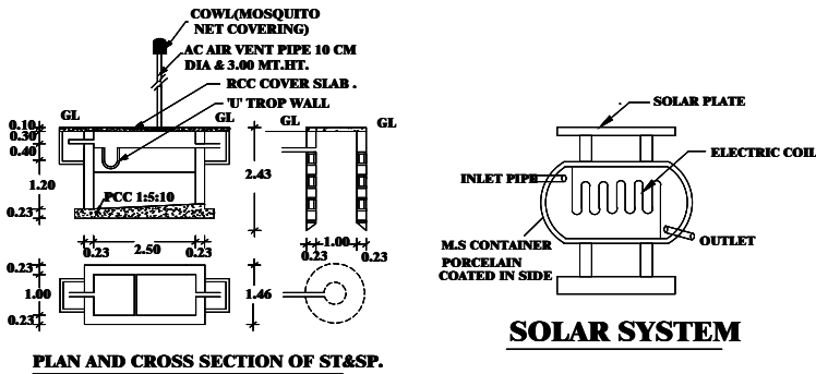
PLAN AND CROSS SECTION OF ST&SP.
