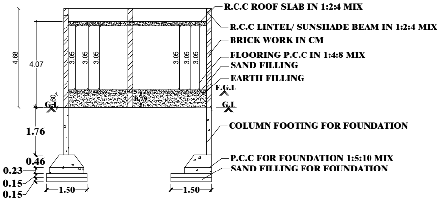
SECTION ON-SD
