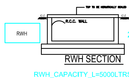
RWH SECTION
