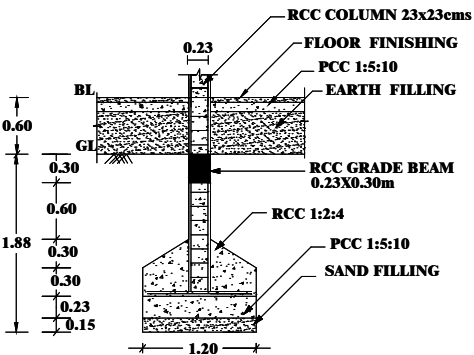
FOUNDATION DETAILS
