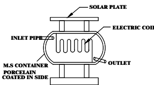
SOLAR SYSTEM
