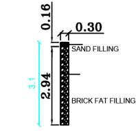
DETAILS OF PERCOLATION PIT RW_H_CAPACITY_L=1000 LTRS
