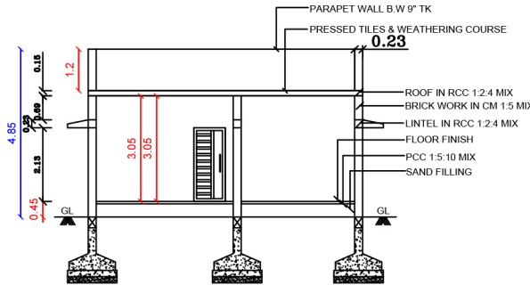
CROSS SECTION AB
