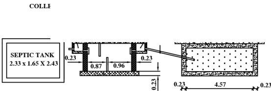
PLAN & SECTION ON SEPTIC TANK & DISP-TRENCH
