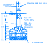
FOUNDATION DETAILS Scale: 1:50
