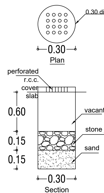
RAIN WATER PERCULATION PIT
