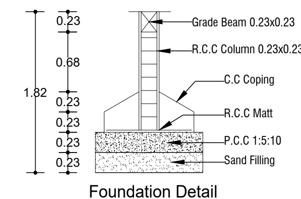
Foundation Detail
