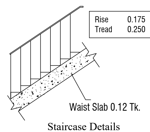
Staircase Details
