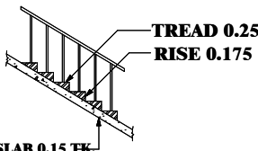
R.C.C WAIST SLAB 0.15 THK STAIR CASE DETAILS
