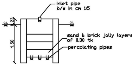
SECTION OF RAIN WATER HARVESTING PIT
