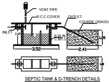
SEPTIC TANK & D-TRENCH DETAILS
