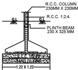
FOUNDATION DETAIL (NOT TO SCALE)
