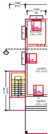
PRO.GOUND FLOOR PLAN
