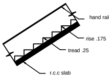
STAIR
