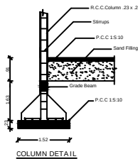
COLUMN DETAIL
