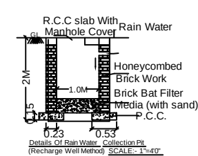
Details of Rain Water Collection Pit (Recharge Well Method) SCALE: 1\"/>
