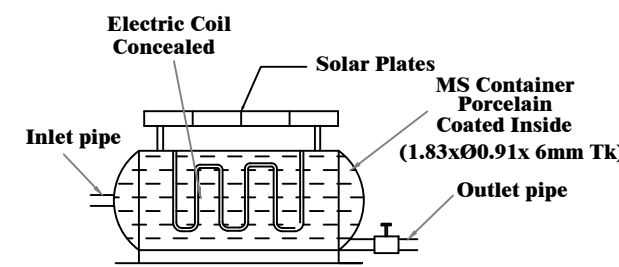
Solar water heater
