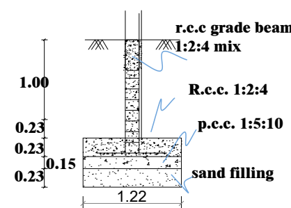
foundation details
