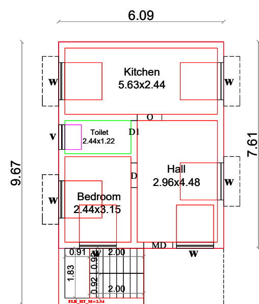
PRO GROUND FLOOR
