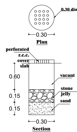
RAIN WATER PERCULATION PIT
