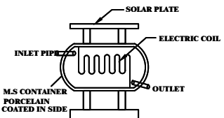
SOLAR SYSTEM
