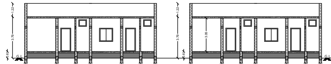
SECTION BLOCK-1 & 2
