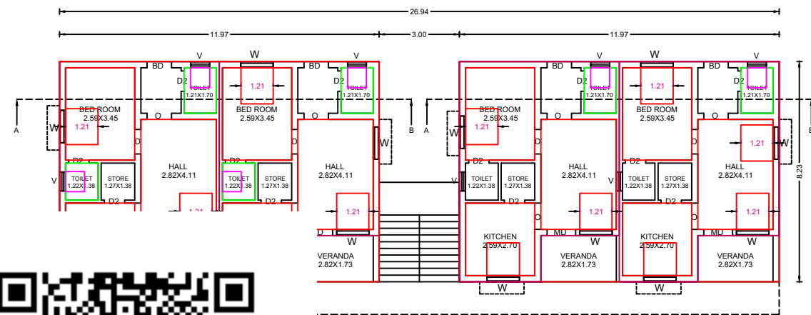
GROUND FLOOR PLAN BLOCK-1 & 2
