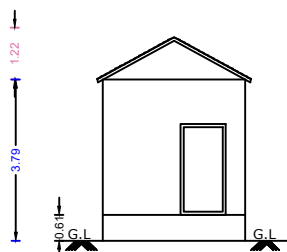
ELAVATION BLOCK-2
