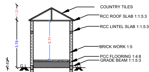
SECTION BLOCK-2
