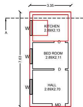
EXI.GROUND FLOOR PLAN BLOCK-2
