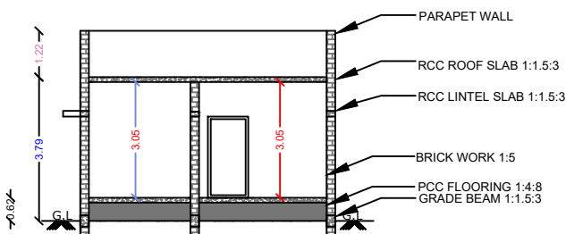
SECTION BLOCK-1
