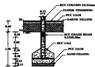
FOUNDATION DETAILS
