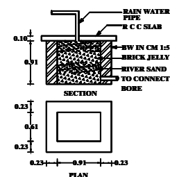
RAIN WATER COLLECTION TANK
