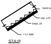
STAIR
