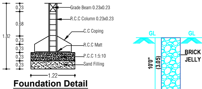
Foundation Detail
