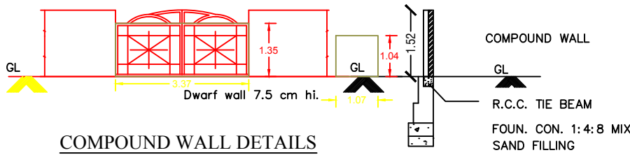
SECTION
