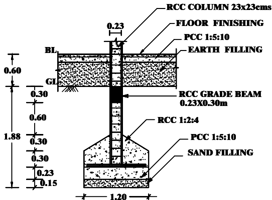
FOUNDATION DETAILS
