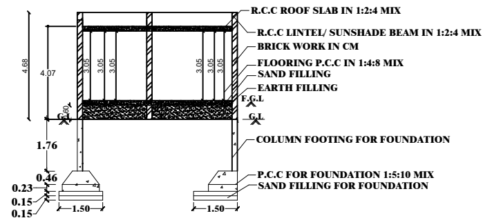
SECTION ON-SD
