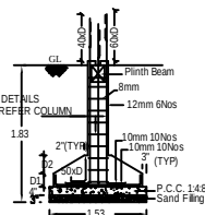
FOUNDATION DETAILS
