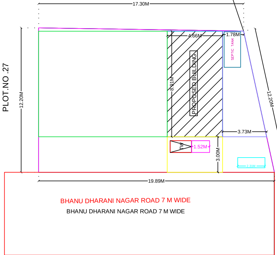
SITE PLAN
