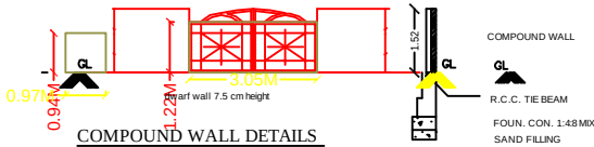
SECTION
