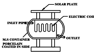
SOLAR SYSTEM
