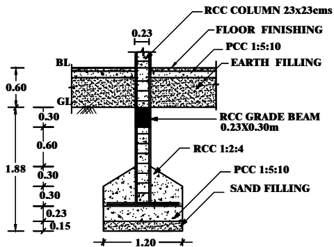
FOUNDATION DETAILS
