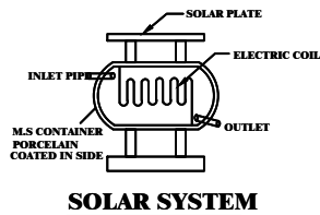
SOLAR SYSTEM
