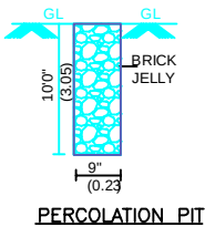
PERCOLATION PIT
