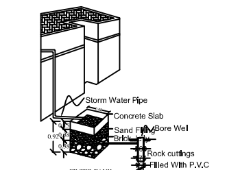
RAIN WATER STORAGE ARRANGEMENTS
