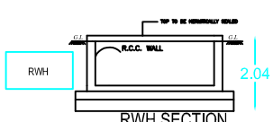
RWH SECTION
