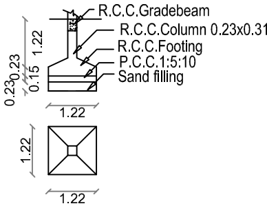
Foundation details
