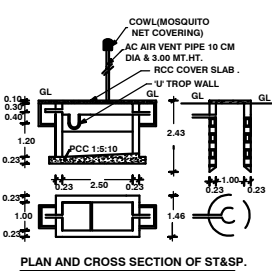
PLAN AND CROSS SECTION OF STAIR.
