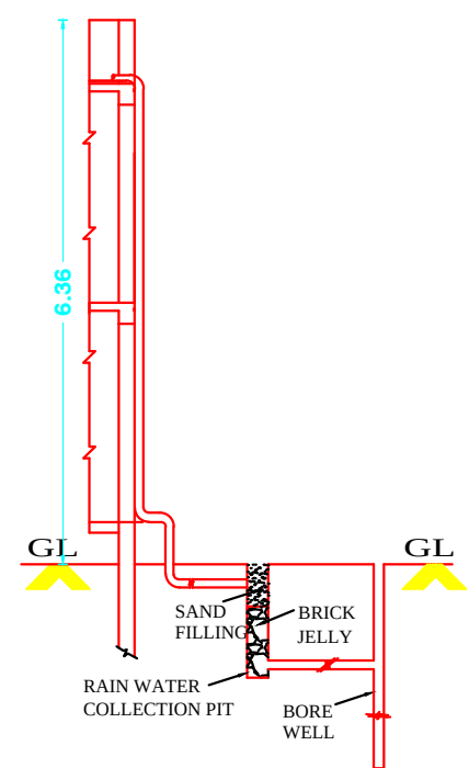
RAIN WATER HARVESTING SYSTEM RWV_CAPACITY_L=1000LTRS
