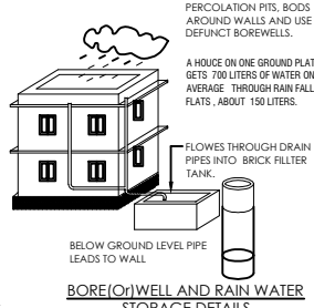
BORE/CUTWELL AND RAIN WATER STORAGE DETAILS
