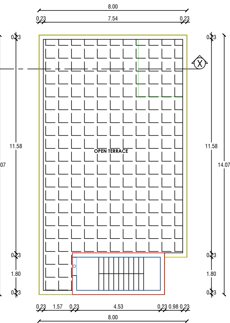
TERRACE FLOOR PLAN (PROPOSED)
