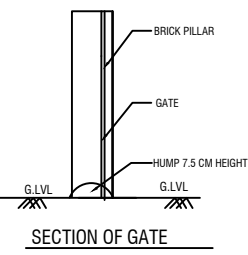
SECTION OF GATE
