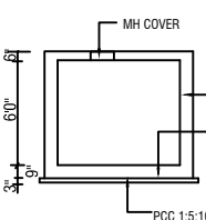
SUMP PLAN (SCIENTIFICALLY CLOSED)
