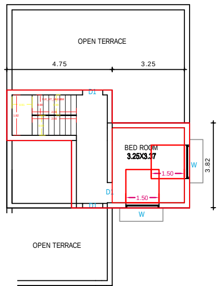
RO FIRST FLOOR PLAN
