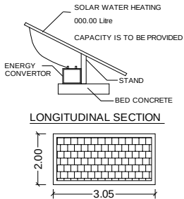
SOLAR SYSTEM
