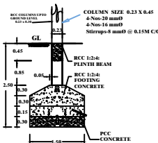
FOUNDATION DETAILS
