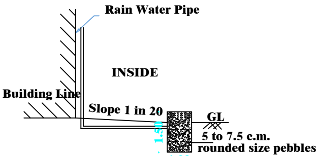
RAINWATER HARVESTING
