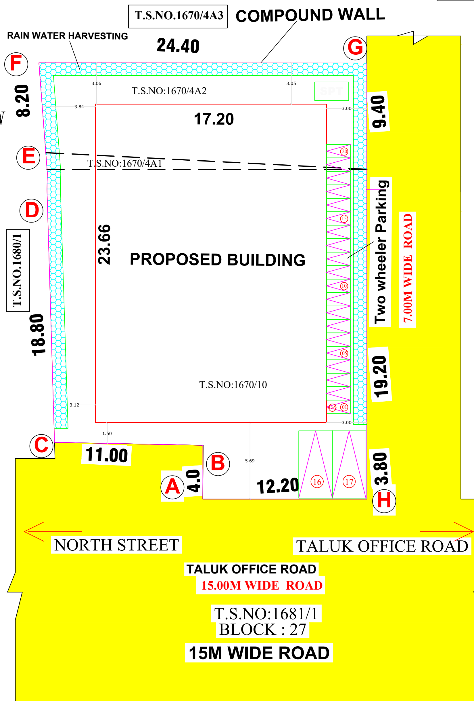
SITE PLAN
