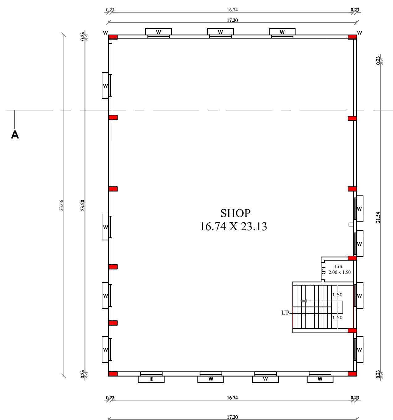
TYPICAL FLOOR PLAN GROUND, FIRST, SECOND FLOOR PLAN
