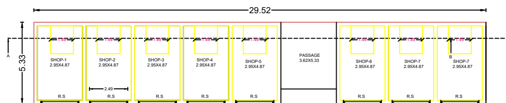
PLAN
