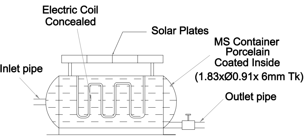
Solar water heater
