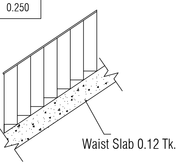
Staircase Details
