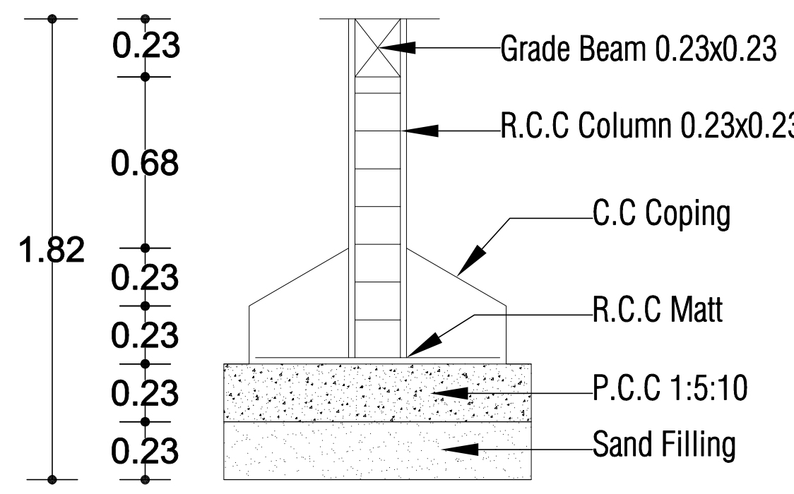
Foundation Detail
