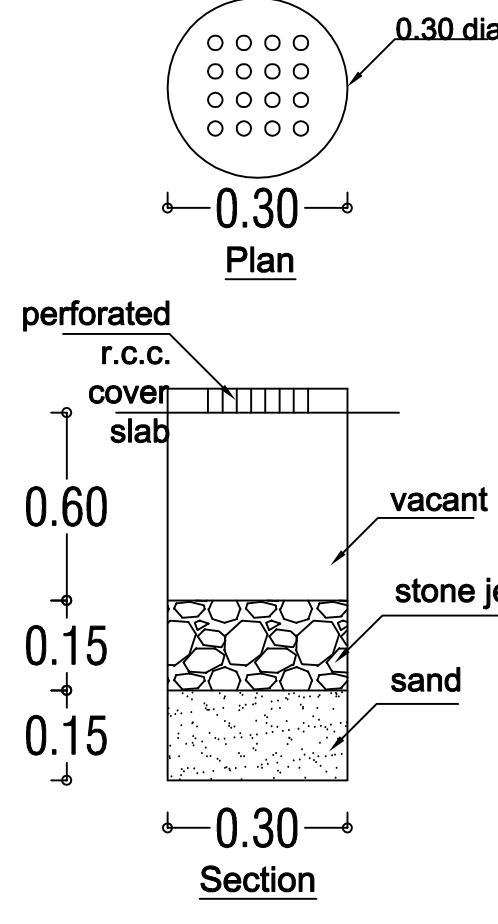
RAIN WATER PERCOLATION PIT
