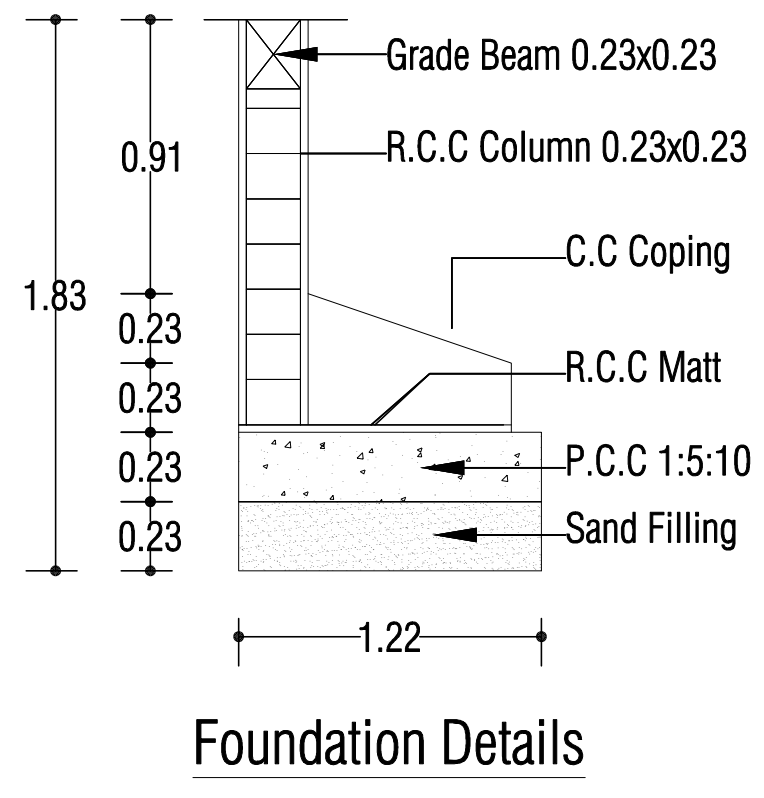
Foundation Details
